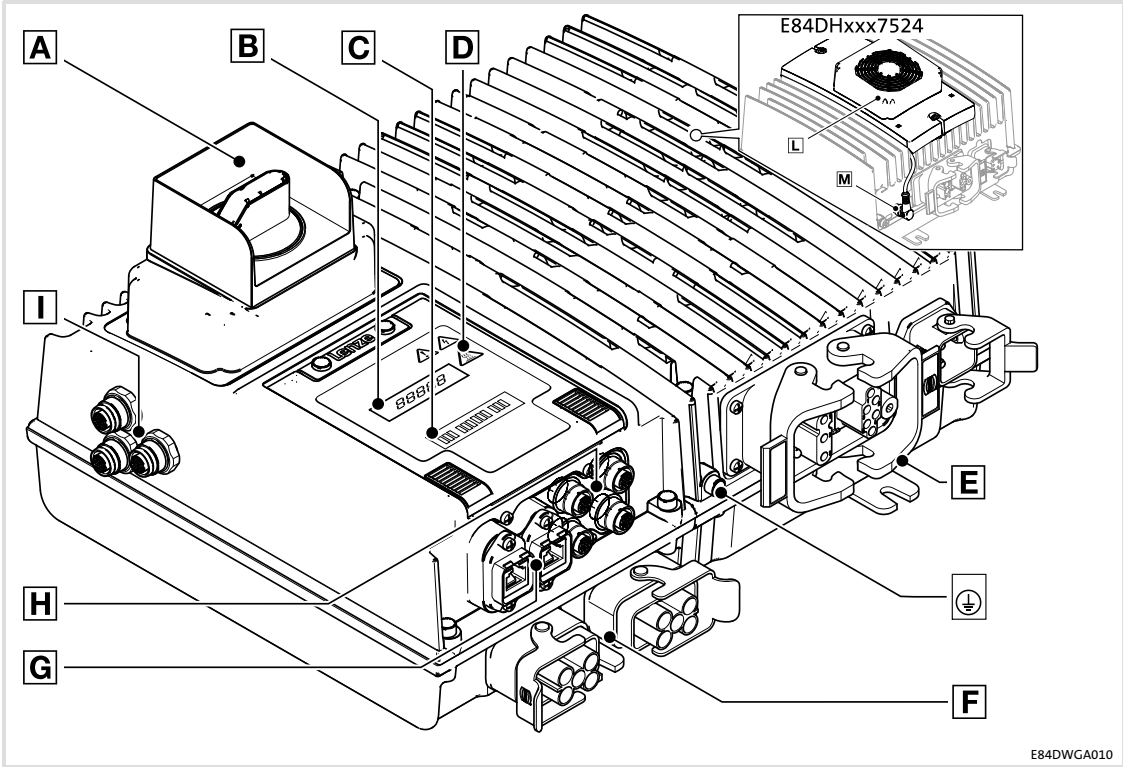
Control elements and overview of connections
