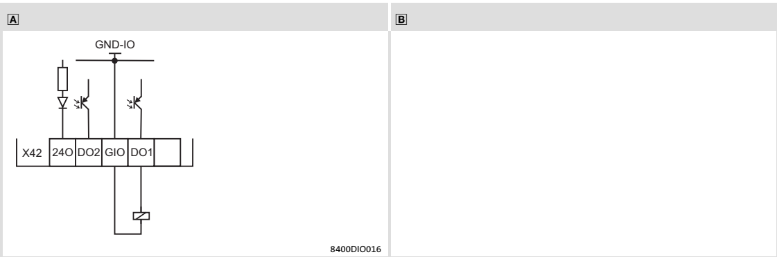
Fig. 7-6 A Digital control (relay, valve, ...) with internal 24 V supply B - X42 Plug for the digital outputs (configured) GIO Ground reference potential for the digital inputs and outputs (GND-IO)
