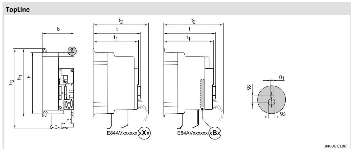
Fig. 5-21 Device dimensions
