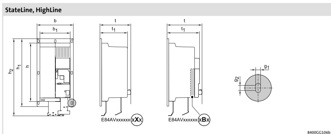
Fig. 5-33 Device dimensions
