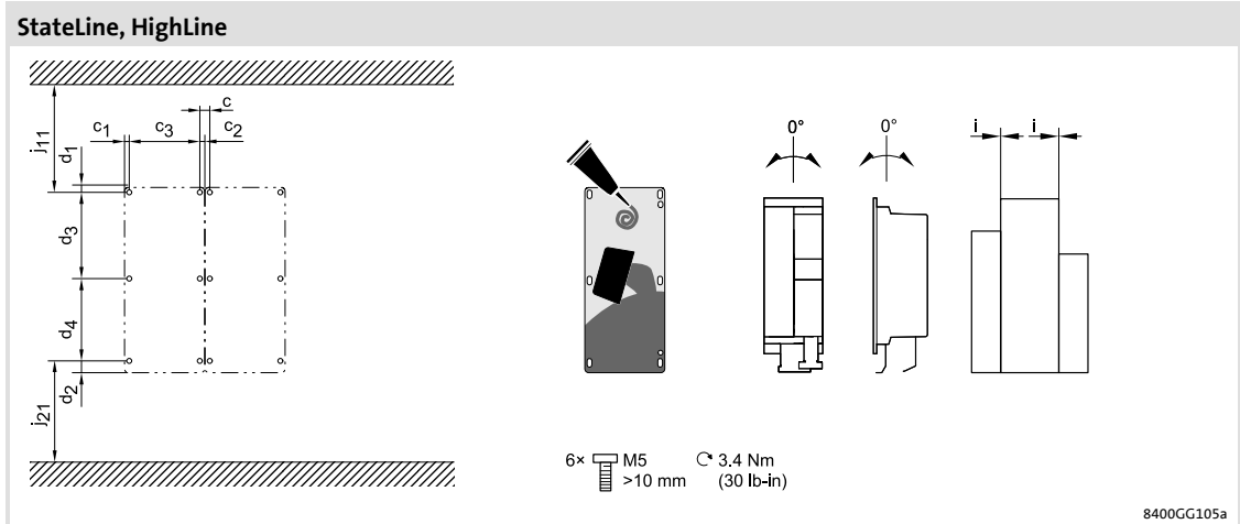
Fig. 5-12 Dimensions for mounting
