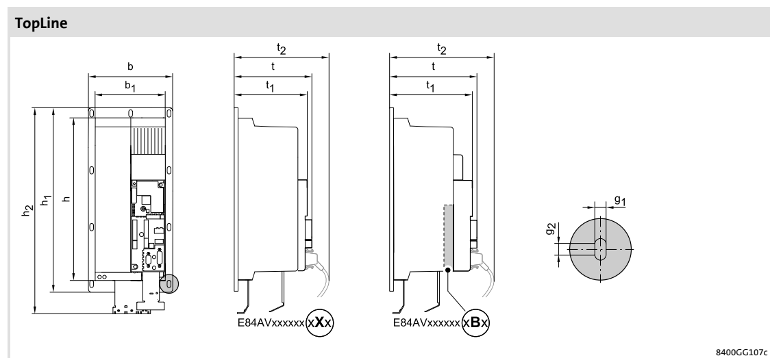
Fig. 5-39 Device dimensions
