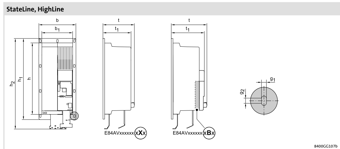
Fig. 5-37 Device dimensions
