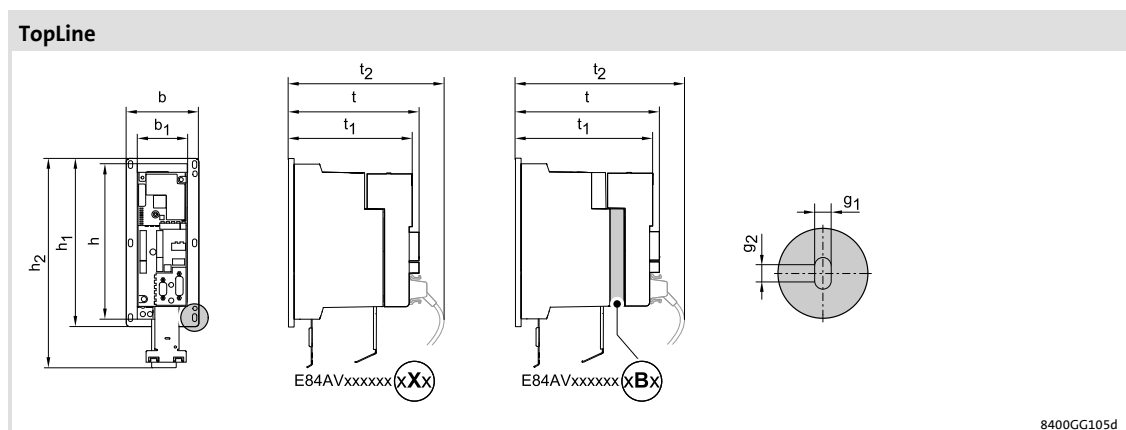
Fig. 5-13 Device dimensions
