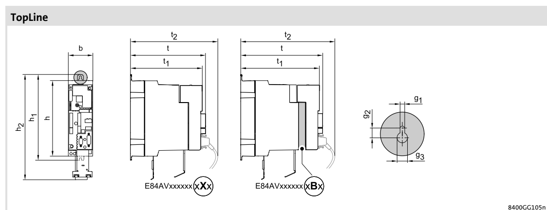
Fig. 5-3 Device dimensions
