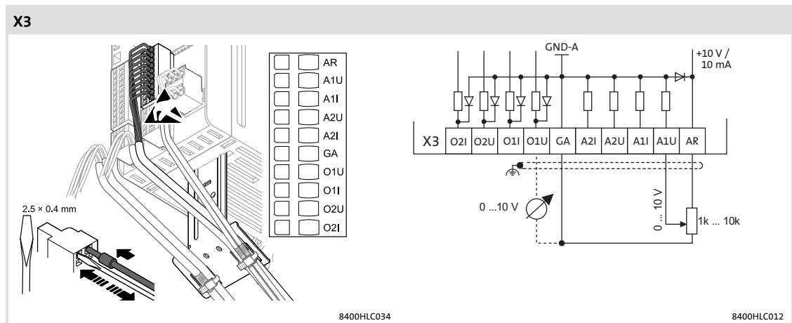
Fig. 6-40 Connection of the analog inputs and outputs
