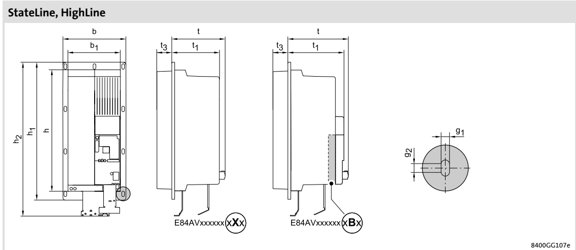
Fig. 5-29 Device dimensions
